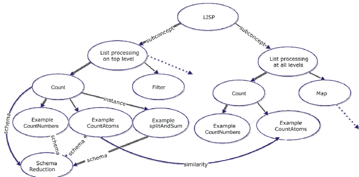
Figure 4. Part of the ALEA domain model for functional list processing.
