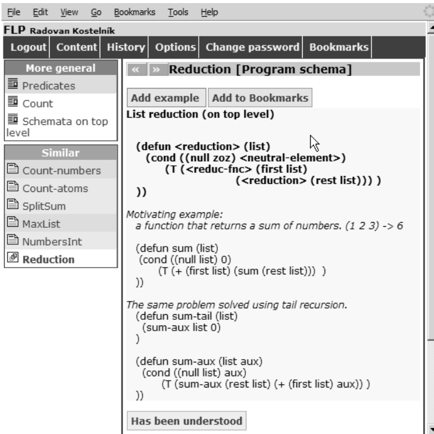
Figure 2. Reduction program schema (the content area of ALEA screen is shown).
