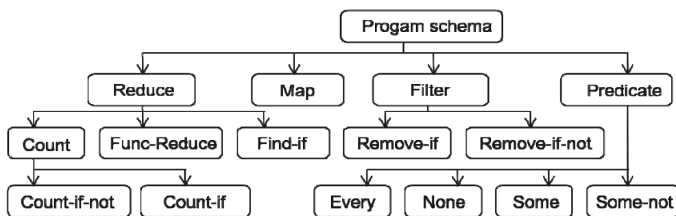
Figure 1 The hierarchy of program schemata for processing of lists
