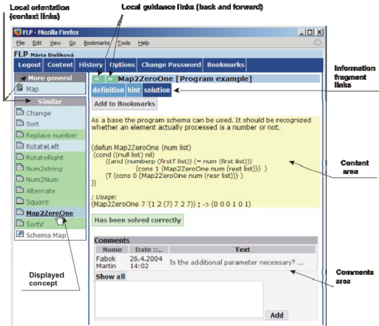
Figure 3. A screen shot from ALEA interface representing a solution of the list mapping programming task.
